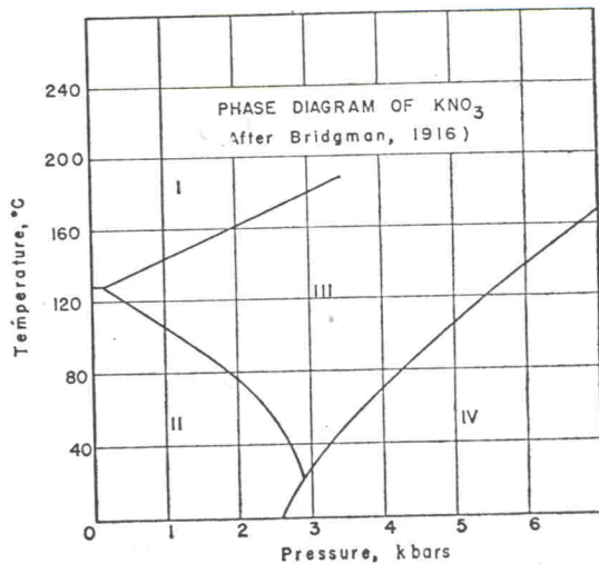
FIG. 1. Phase diagram of \text{KNO}_3 (after BRIDGMAN (6) ).
